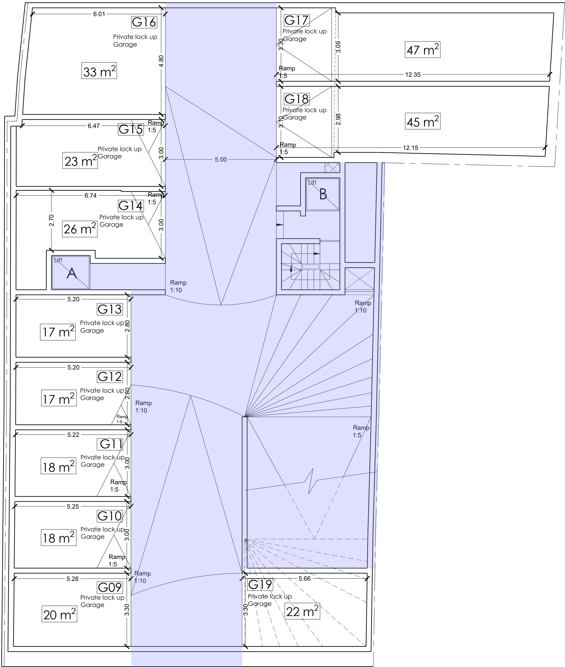
Lower Basement Floor (Level 1)
